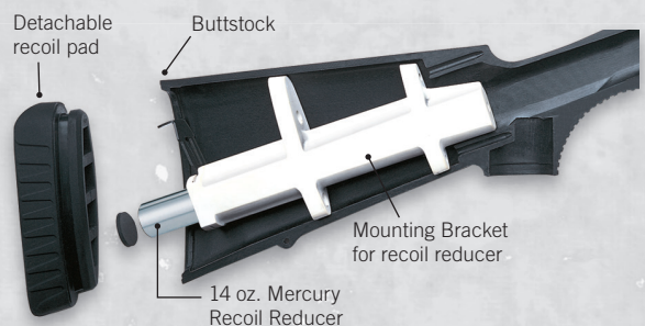
Item # 80208 Nova Recoil Reducer Package Includes the mercury recoil reducer and bracket for easy installaton.
